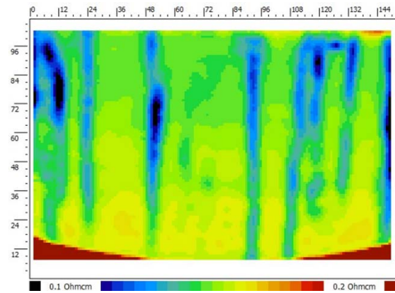
Figure 9: Resistivity mapping of a side of a square brick of the ingot with 10 % refined material.
