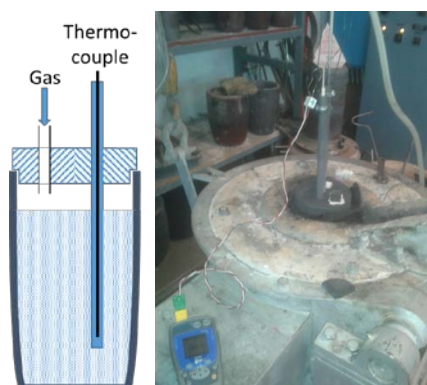
Figure 4: Schematic of the melting and separation setup on the left hand side and a photo of the experimental setup at the right. The inner diameter of the crucible is 150 mm and about 300 mm inner height.
