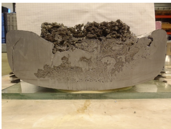
Figure 3: Cut plane of the first ingot. In addition to the particles on top, there are also large amounts of oxides embedded inside the ingot.
