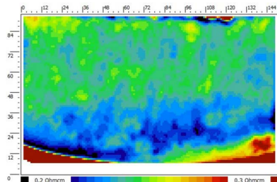
Figure 10: Resistivity mapping of a side of a square brick of the ingot with 100 % refined material.
