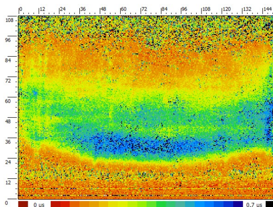
Figure 10: Lifetime mapping of the side of the 10 % ingot.
