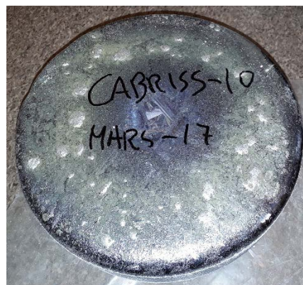
Figure 5: Photo of the ingot with 10 % refined material and 90 % poly-Si.
