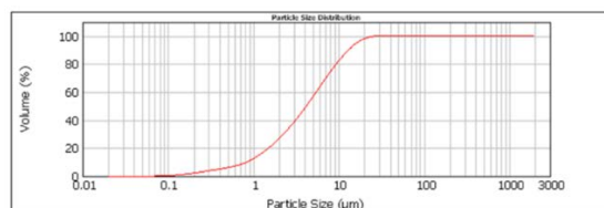
Figure 1: Size distribution of the silicon powder from ReSiTec.
