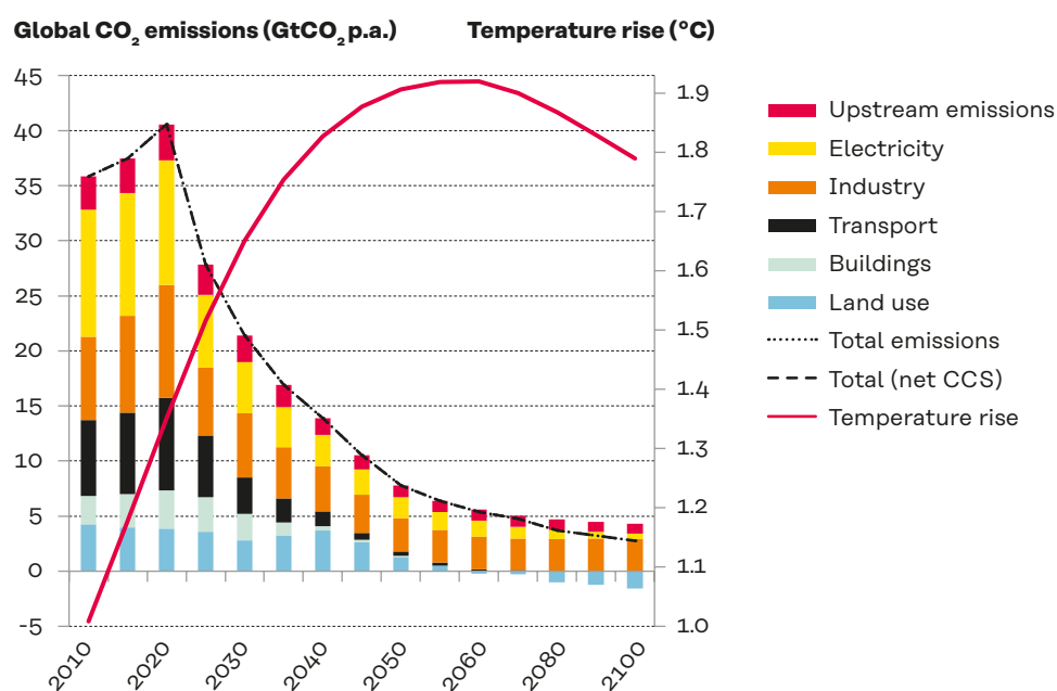
Figure 31: CO 2 emissions trajectory (no CCS or NETs, and slow coal phase-out)
