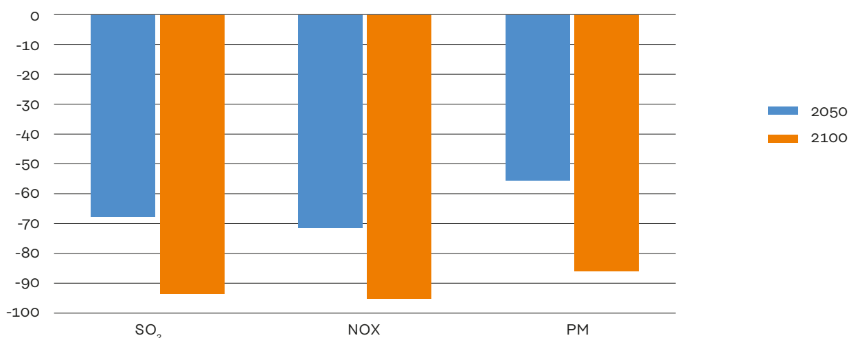
Figure 28: EU air pollutant emissions in the central scenario over the period 2015-2100
