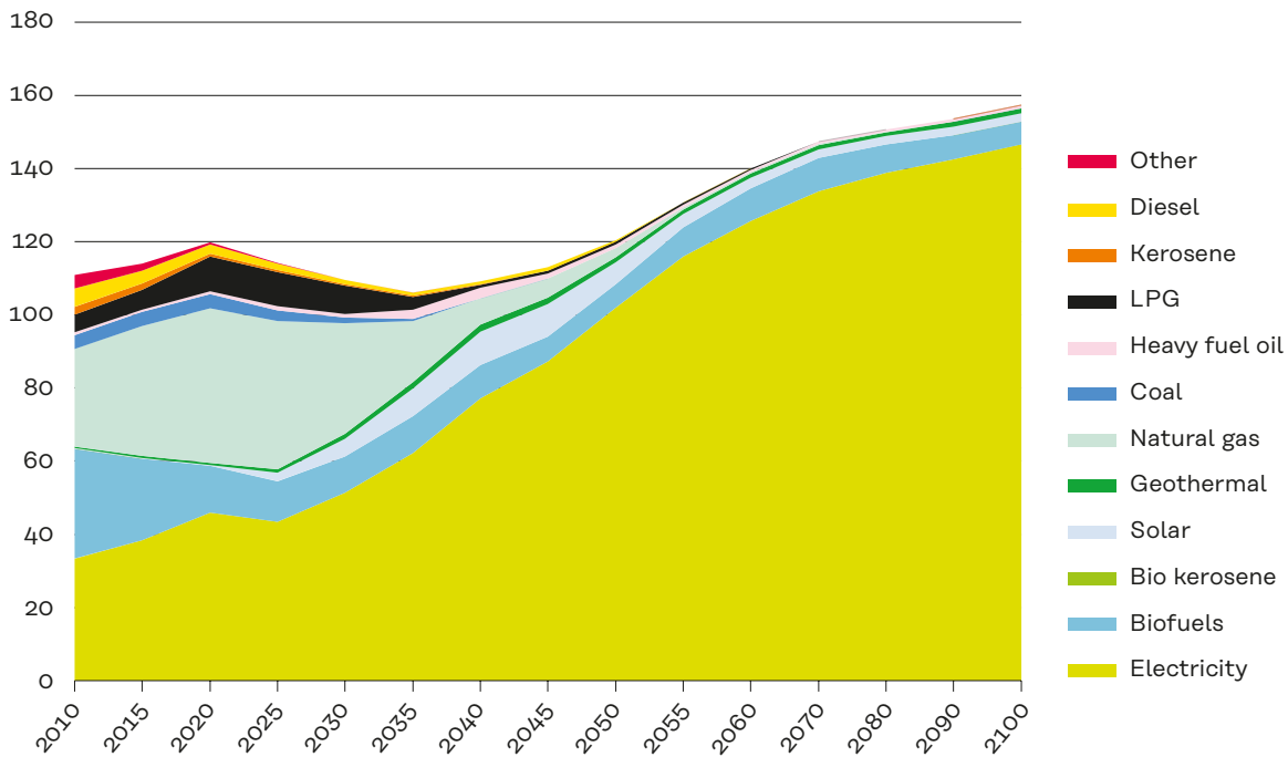
Figure 19: Energy consumption in transport sector (central scenario)
