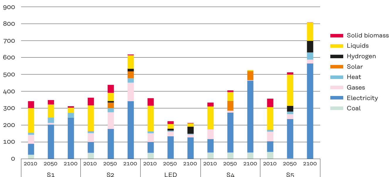
Figure 13: Global final energy consumption
